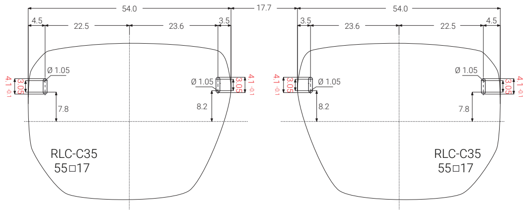
RLC-C35 4.5_3.5_3.05
