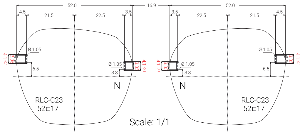
RLC-C36 4.5_3.5_3.05
